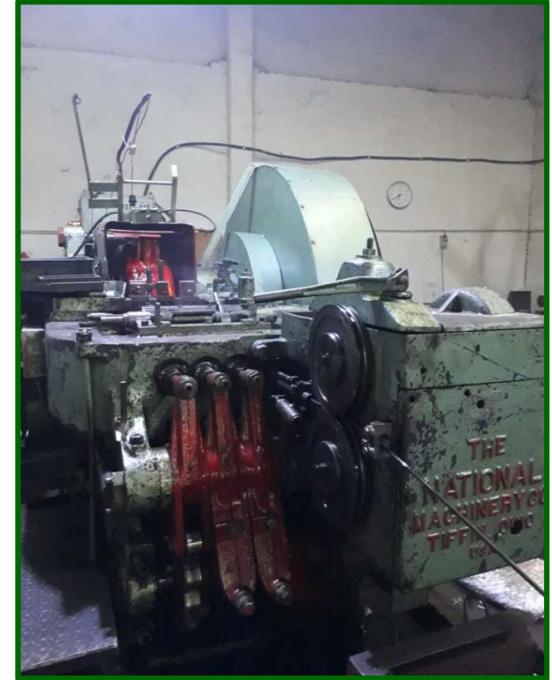
4 Station, 3 die, Bolt Former Make: Naitonal, USA
